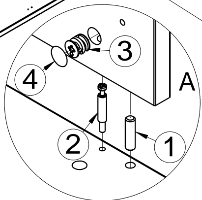
Assembling back
