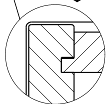
Assembling back
